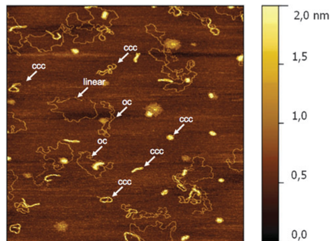
FIG. 2. AFM image of the 7-year-stored plasmid DNA. The AFM image shows ccc plasmid DNA of different degrees of condensation and oc forms (without linear forms, chromosomal DNA aggregates, or other contaminants). The figure shows an AFM image with an edge size of 3\ \mu\text{m} . The altitude of the DNA above the surface (in nm) is shown by different colors as indicated on the bar on the right-hand side of the AFM image. AFM, atomic force microscopy; ccc, covalently closed circular; oc, open circular. Color images available online at www.liebertpub.com/humc
